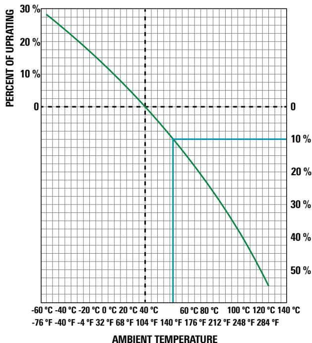
FIGURE 3. Temperature derating curve.
