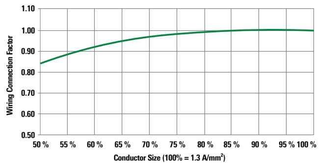
FIGURE 4. Thermal correction factor.
